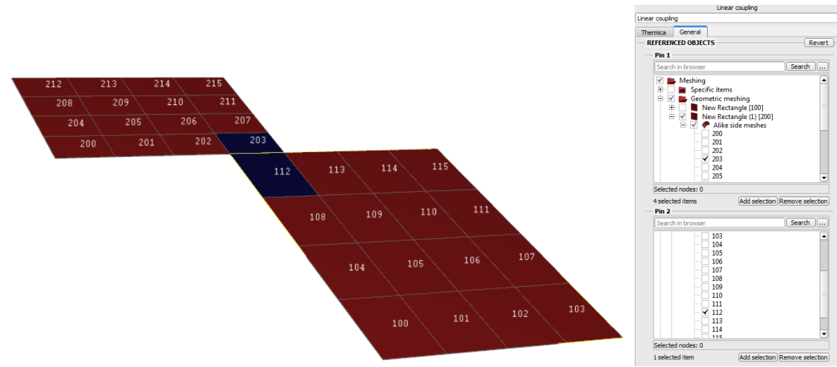
Creation of a linear coupling from the GUI between node 203 and 112
