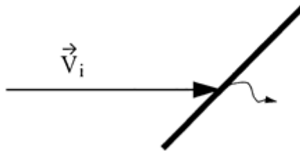
Figure 2.1-2 Absorption
