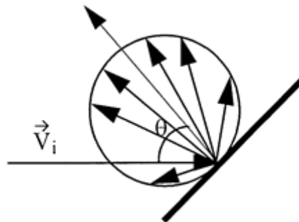
Figure 2.1-4 Diffuse reflection
